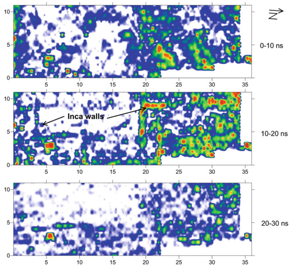
Ground-Penetrating Radar, Fig. 3 Amplitude slice maps displayed in two-way radar travel time measured in nanoseconds (ns). Each 10 ns interval represents approximately 40 cm of depth. The horizontal slice representing 10–20 ns shows distinct high-amplitude walls, produced from buried Inca structures in highland Ecuador
