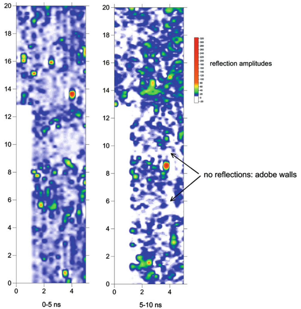
Ground-Penetrating Radar, Fig. 8 Amplitude slice map of the adobe walls shown in Fig. 7. The walls are shown in white as areas of no reflection, while random stones or layers of adobe melt adjacent to the walls produce high-amplitude reflections. These are Hohokam walls in Tucson, Arizona, USA
