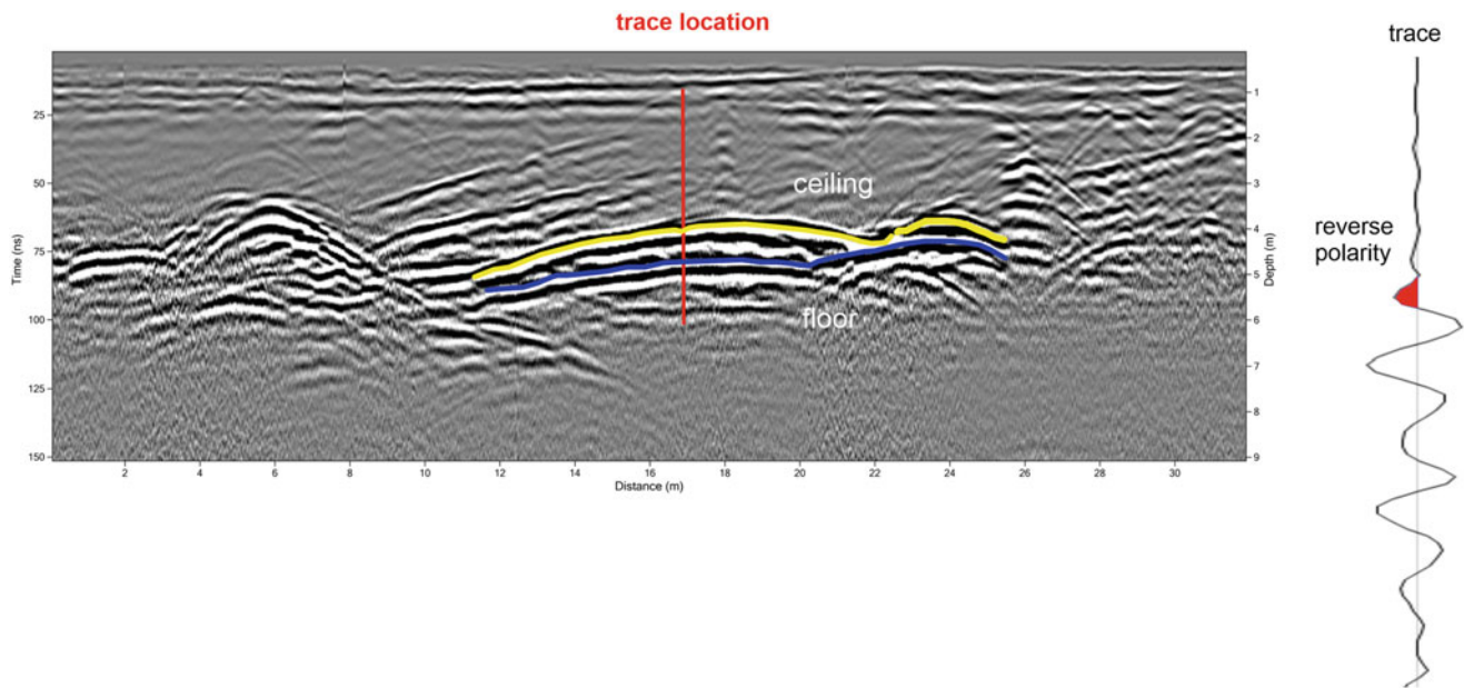
Ground-Penetrating Radar, Fig. 11 Interpretation of one GPR reflection profile from a cave in Spain showing the ceiling and floor interfaces that were “picked” and their depths exported as digital values. The ceiling in this profile was identified by the reverse polarity reflection
