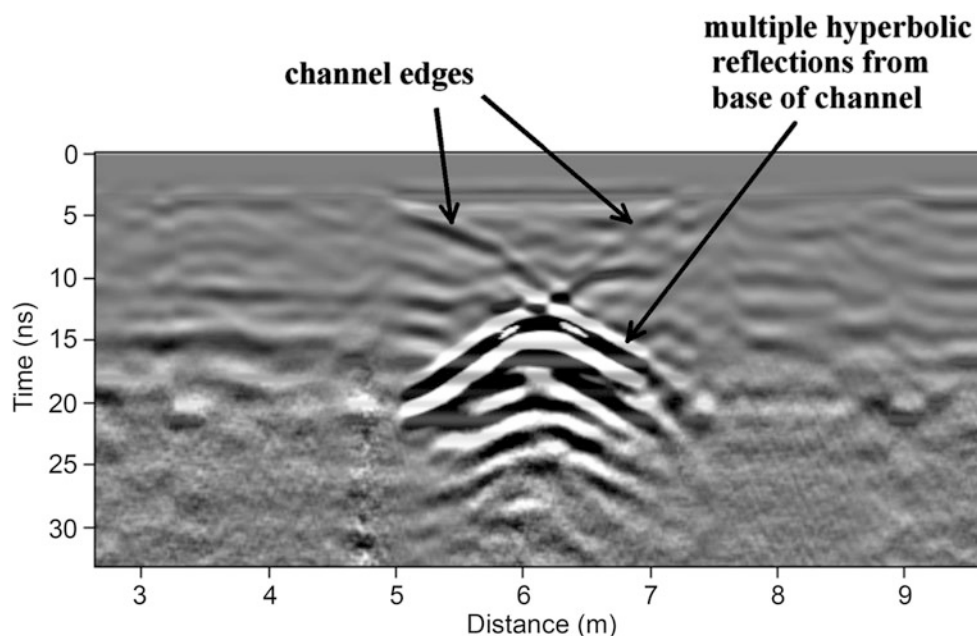
Ground-Penetrating Radar, Fig. 5 Reflection profile from a buried channel that demonstrates reflections similar to those modeled in Fig. 4. The channel edges are of very low amplitude, while a very high-amplitude series of hyperbolic reflections are recorded from the base of the channel, which are recorded as high amplitude due to the upwardly convex surface that focuses energy. This profile was collected over an early agricultural age canal near Tucson, Arizona, USA
