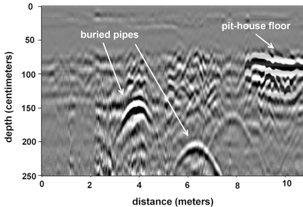
Ground-Penetrating Radar, Fig. 2 A reflection profile 11 m long displaying reflections to a depth of 250 cm. Two hyperbolic reflections from buried pipes are point source reflections, and a distinct planar reflection was produced from a buried house floor. This profile was collected in a water pipeline right-of-way near Alamogordo, New Mexico, USA
