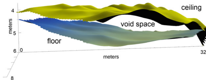
Ground-Penetrating Radar, Fig. 12 Exported depth values from the “picking” of the ceiling and floor reflections of the cave were adjusted for correct depth using velocity measurements and placed into a
