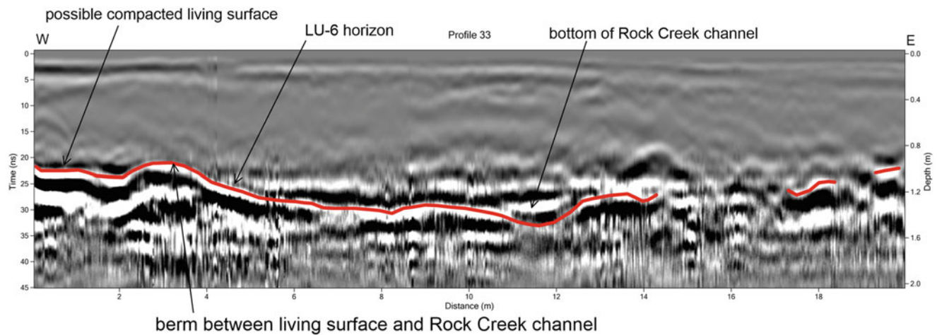
Ground-Penetrating Radar, Fig. 9 The “picking” of one interface in the ground along one reflection produces digital data of its depth, which can then be exported, along with similar data from adjacent profiles for
